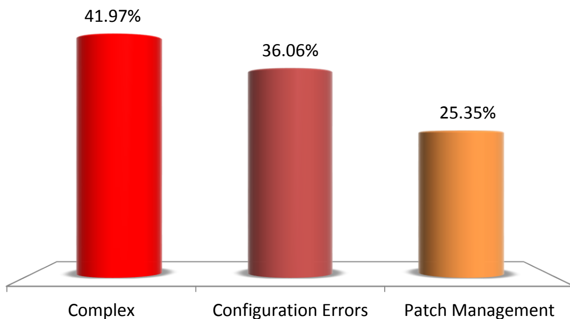
Fig. 18. Vulnerability Types
